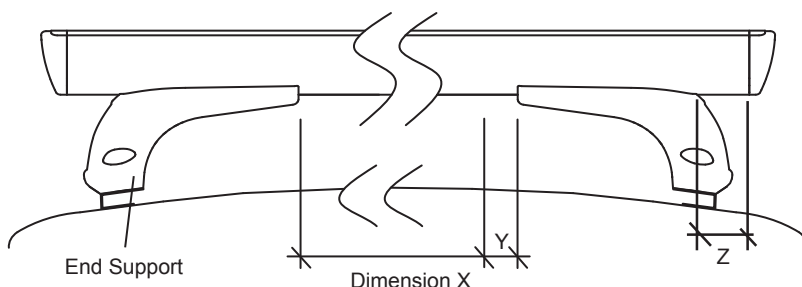
Fig. 5 (Measured between End Supports for H/D type bar (Dim. X) or from End Support to edge of cutout for Sports bar (Y))
